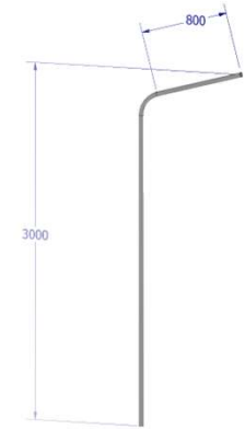
780211 Structure is Stainless Steel 316L.
